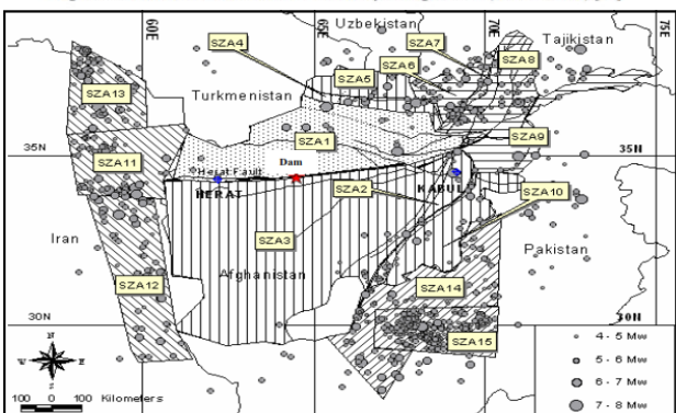
Figure 2-5: Seismogenic zoning, scenario A [28]
