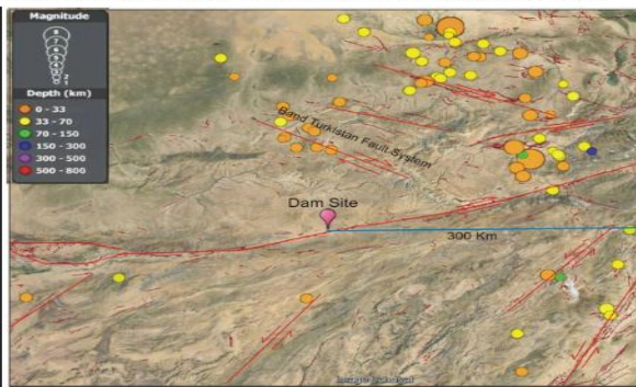
Figure 2-4: Earthquake distribution and fault location around Dam Site
