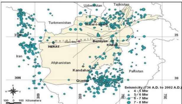
Figure 2-3: Historical and instrumental seismicity of Afghanistan (734-2002 AD) [28]
