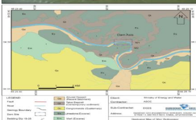
Map 1-2: Geological map of proposed dam area
