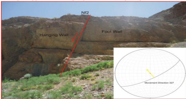
Figure 1- 13: NF2 fault view to NE
