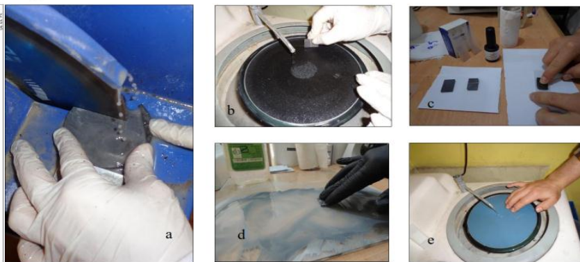
Figure 1-17: a) Cutting, b) initial lapping, c) mounting to glass slide, d) removal of excess mineral, e) final lapping
