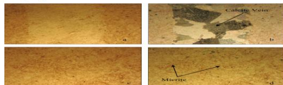
Figure 1-20: Shows microscopic pictures of sample (a,b) shows calcite vein PPL and XPL magnification 40x. (c,d) shows micrite (very fine calcite minerals) PPL and XPL magnification 40x.
