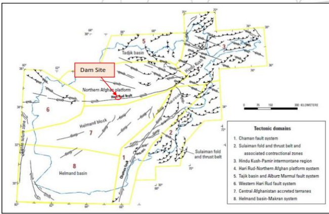
Figure 1-11: Schematic map of probable and possible Quaternary faults in Afghanistan. Each domain is numbered as discussed in the text and boundaries are shown in yellow. Solid lines with arrows denote strike-slip faults, arrows show directions of movement. [3]
