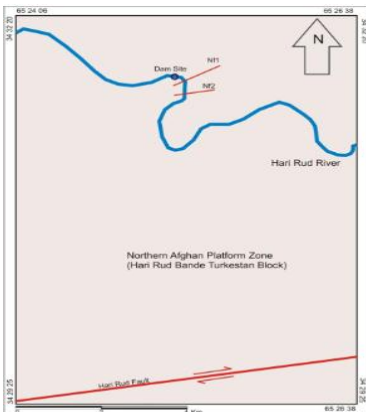
Figure 1-15: Schematic Fault Map of study area
