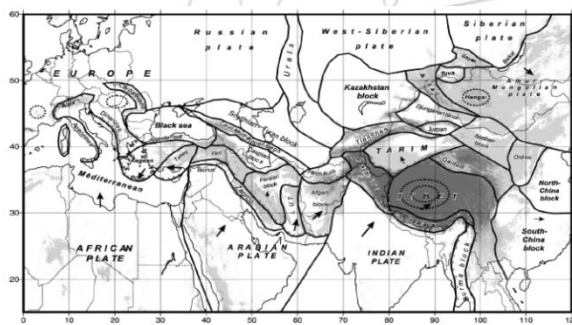
Figure 2-1: Surface topography and generalized structure of the Alpine-Himalayan belt [11]
