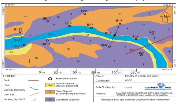
Map 3-1: Location and distribution of boreholes on geological map
