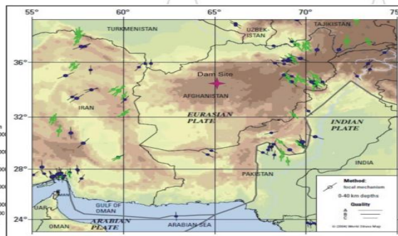
Figure 2-2: Map showing the location of Afghanistan and tectonic features [11]
