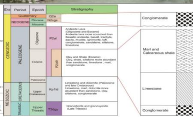
Figure 1-7: Stratigraphic column [7]
