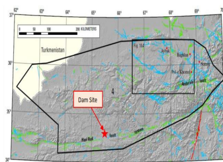
Figure 1-12: Tectonic domain 4—Hari Rud-Northern Afghan platform system outlined in black [5]
