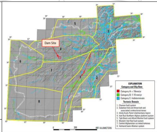
Figure 1-10: Probable and possible Quaternary faults and eight tectonic domains [3]
