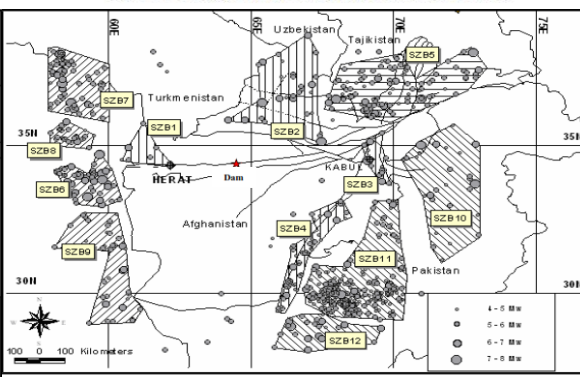
Figure 2-6: Seismogenic zoning, scenario B [28]
